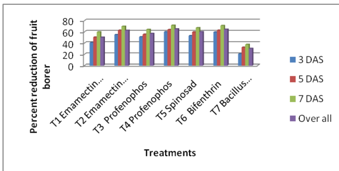
Fig. 1: Efficacy of insecticides against fruit borer ( Helicoverpa armigera ) after first spray
