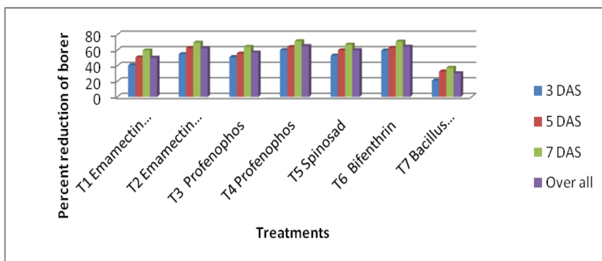
Fig. 2: Efficacy of insecticides against fruit borer ( Helicoverpa armigera ) after second spray
