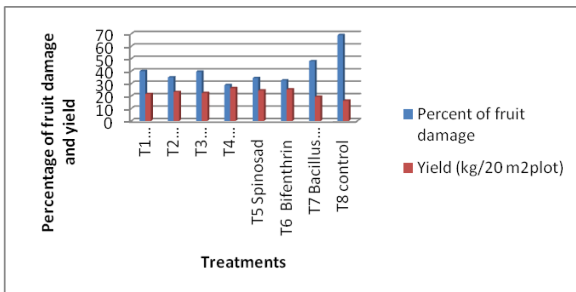
Fig. 3: effect of pesticides on fruit damage and yield
